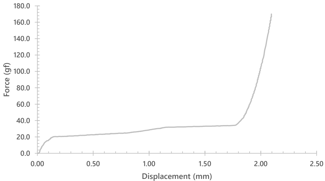
Kailh Low Profile Purple Iris (Upstroke)
